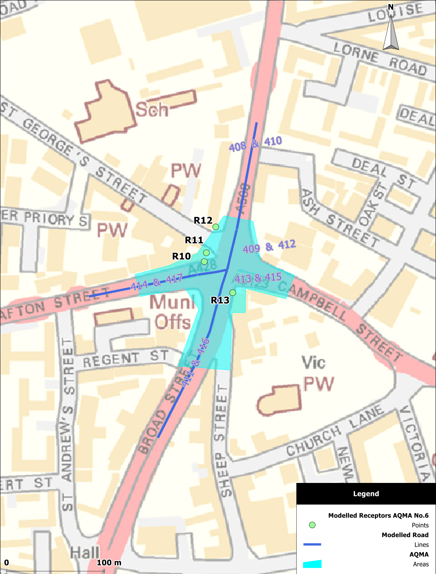
Figure 9.10: Local Operational Impacts - Northampton AQMA No.6, Campbell Square
