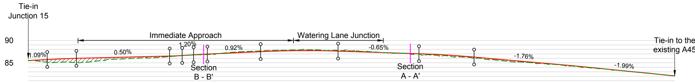
A45 NORTH - MAINLINE CENTRELINE - LONGSECTION SCALE: H 1:2500, V 1:500. DATUM: 80.000
